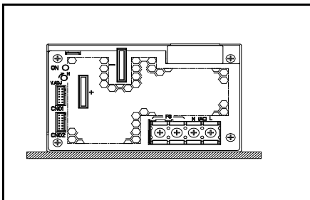
MOUNTING D
