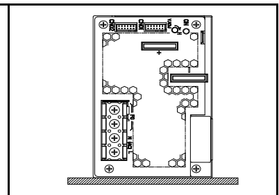
MOUNTING C
