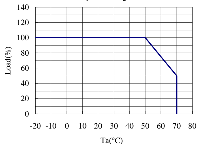
Output Derating Curve
